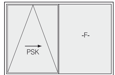
Parallel slide and tilt patio door, left moving door, right fixed pane.
