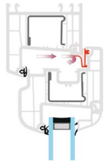
Closed ventilation position for increasing air pressure.
